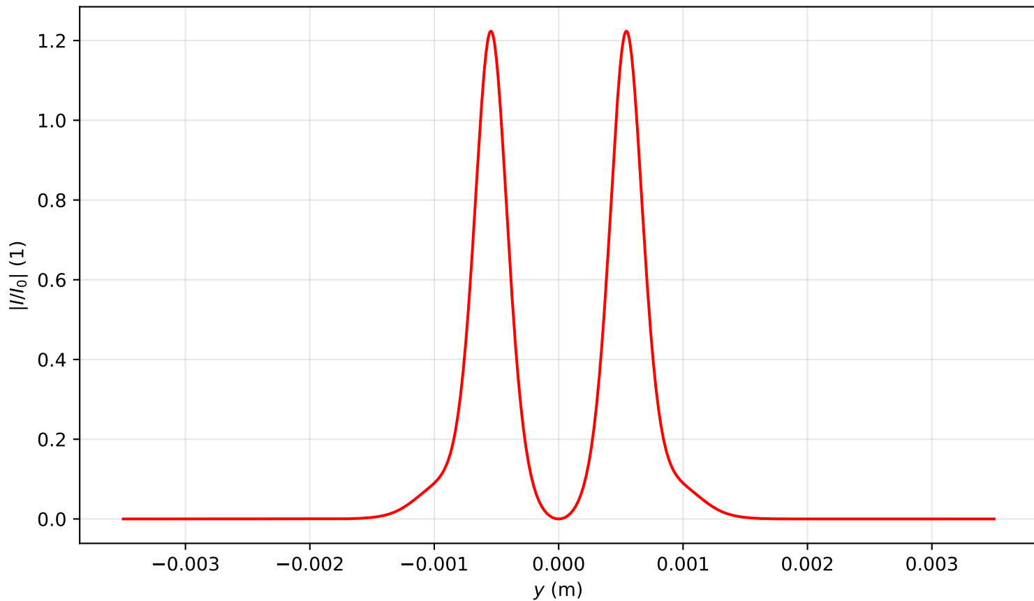
Intensity profile I(x=0, y, z=0.637)/I_0 , P_{in}=6.0P_{cr} , artificial time
